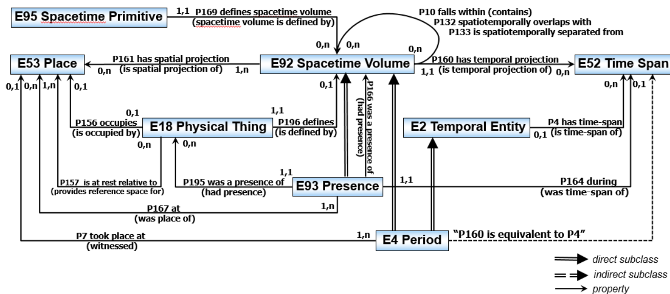
Figure 6: reasoning with spacetime volumes
