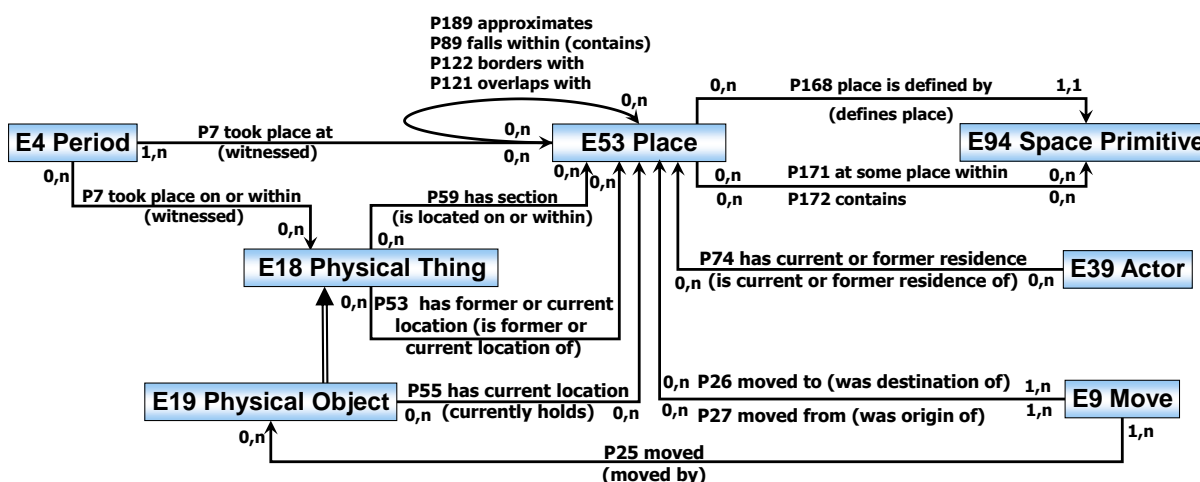
Figure 4: reasoning about spatial information
