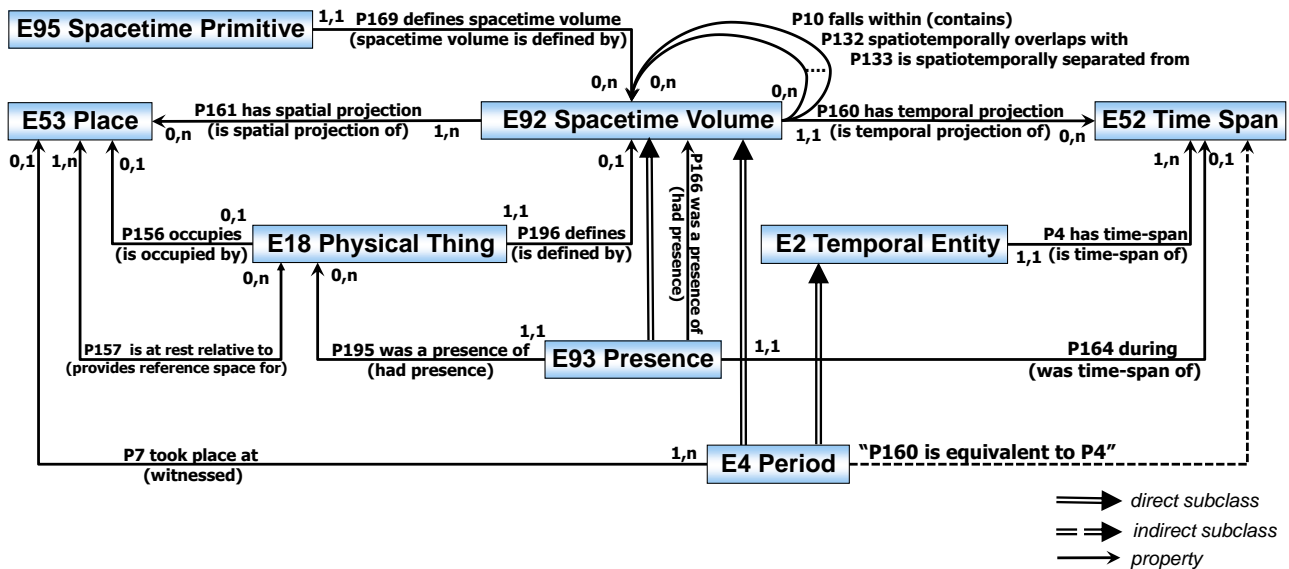
fig. 5 reasoning with spacetime volumes
