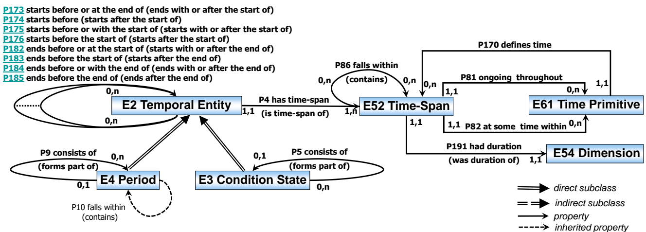
fig. 4 reasoning about temporal information
