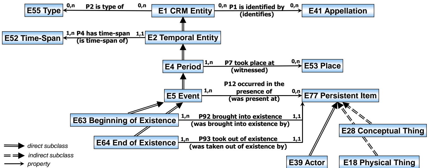
figure 1: properties of basic concepts
